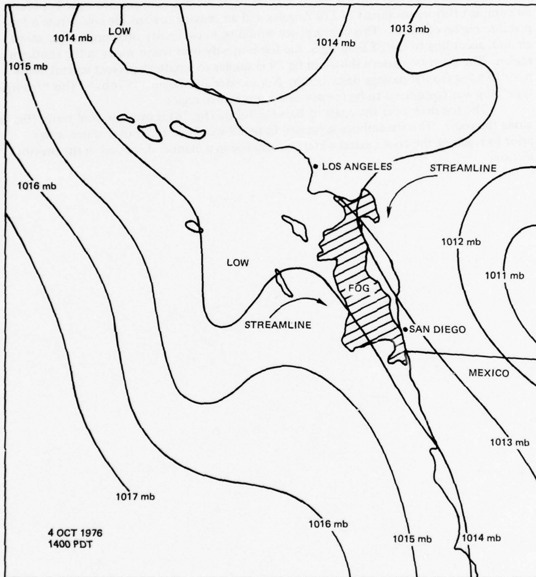
Figure 29. Surface, synoptic pressure pattern with outline of fog patch taken from fig 28.
